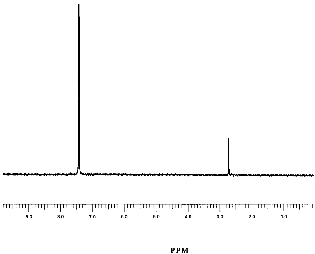
Figure 1: Proton decoupled ^3\text{H} NMR ( \text{CDCl}_3 ) of 1b.
